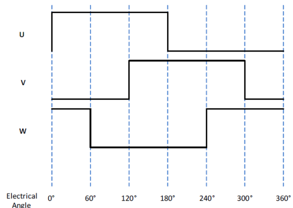
Figure 8: UVW - Output pattern over 360°.
