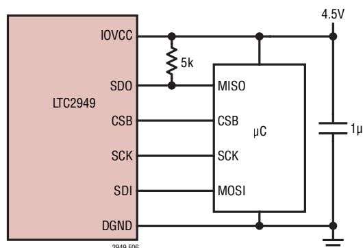
Figure 6. 4-Wire SPI External Connections
