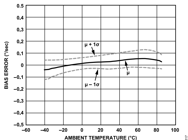
Figure 17. ADIS16477-3 Gyroscope Bias Error vs. Ambient Temperature
