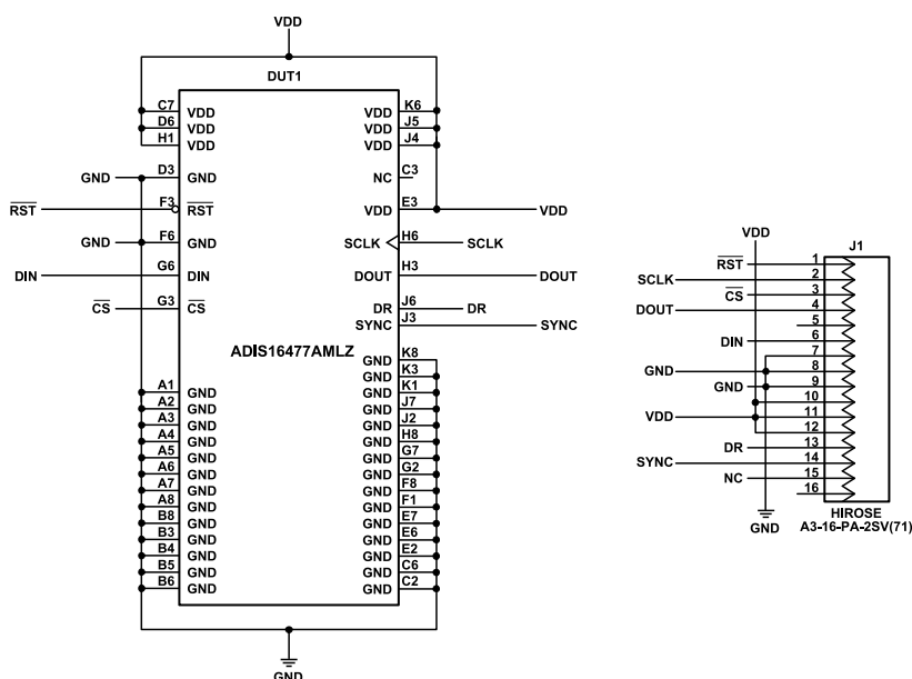
Figure 53. Breakout Board Schematic
