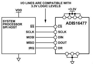
Figure 25. Electrical Connection Diagram
