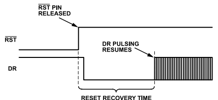
Figure 29. Data Ready Response During Reset ( \bar{RST} = 0 ) Recovery
