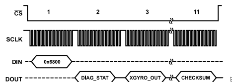
Figure 31. Burst Read Sequence
