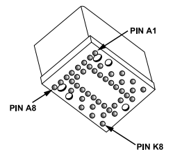
Figure 7. Pin Assignments, Package Level View
