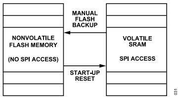
Figure 35. SRAM and Flash Memory Diagram
